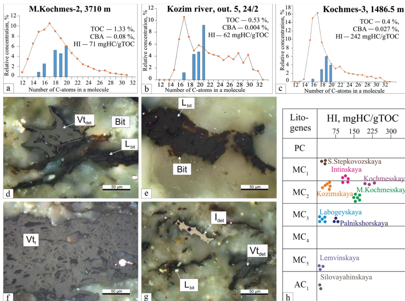
Fig. 2. Histograms of normal and isoprenoid alkanes (a–c) distribution, examples of organic matter inclusions (d–g) and changes in the hydrogen index (h – HI) in P 1 ar rocks (d – Bergantymylkskaya-1 well, depth of 2000.1 m, sample 5-1a; e – Padimeyskaya-1 well, depth 1402.1 m, sample 2-2; f – Padimeyskaya-1 well, depth 1415.2 m, sample 4-4; g – Padimeyskaya-1 well, depth 1414.9 m, sample 4-1; polished sections, reflected light, oil immersion, x50. L bit – bituminite (liptinite group); Vt I – telinite, Vt det – vitrodetrinite (vitrinite group); I det – inertodetrinite (inertinite group); Bit – bitum. Compiled with additions for [6]
