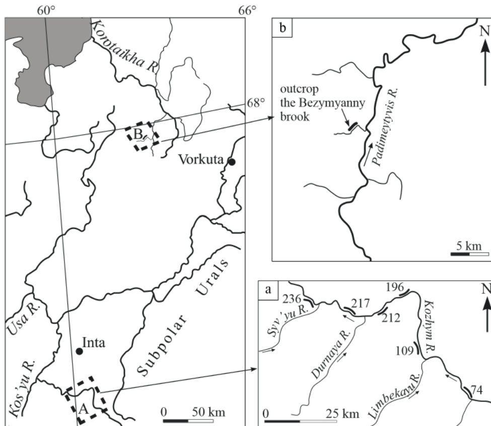
Fig. 1. Scheme of the location of the studied sections: a — western slope of the Subpolar Urals: the Kozhym River (outcrops 74, 109, 212, 196, 217, 236); b — outcrop along the Bezymyanny brook (Chernov Uplift)
